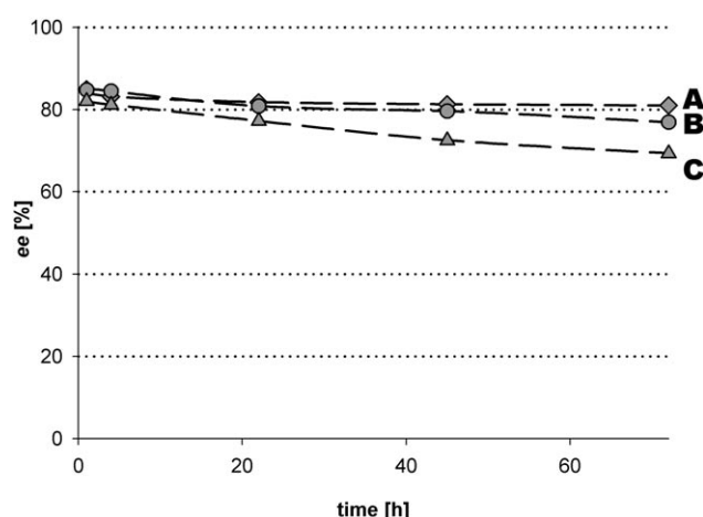
Figure 5. The ees in the MeHNL -catalyzed synthesis of hexanal cyanohydrin. A : free MeHNL , B : MeHNL aqua gel, C : MeHNL -CLEA. Racemisation rates upon the catalysis of HbHNL and PaHNL (free enzyme and aqua gel) were in the range presented here for MeHNL .
